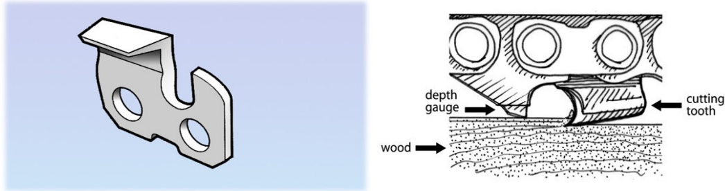
Cutter and depth gauge.
