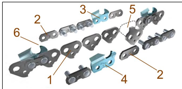
Chain parts numbered.
