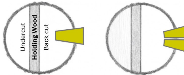
Top view of wedges.
