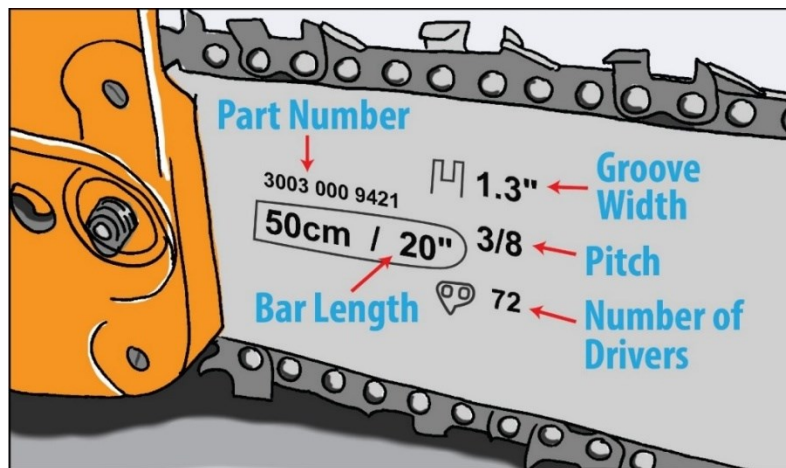
Bar markings.
