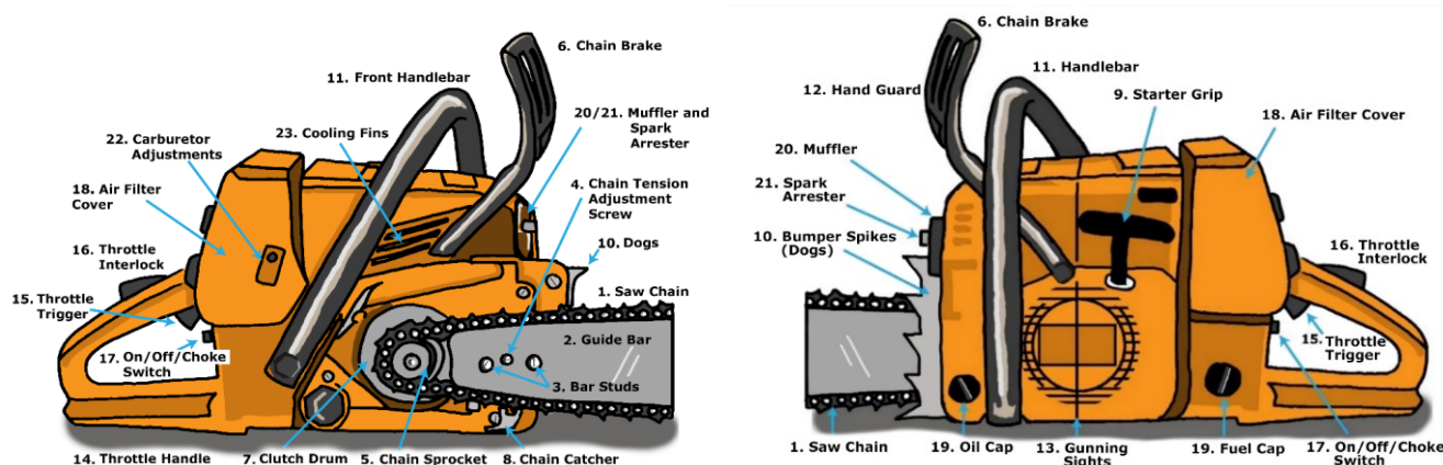
Chainsaw parts numbered.
