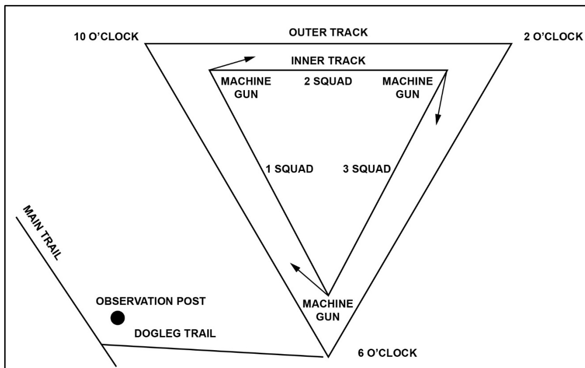
Figure 5-3. Track plan
